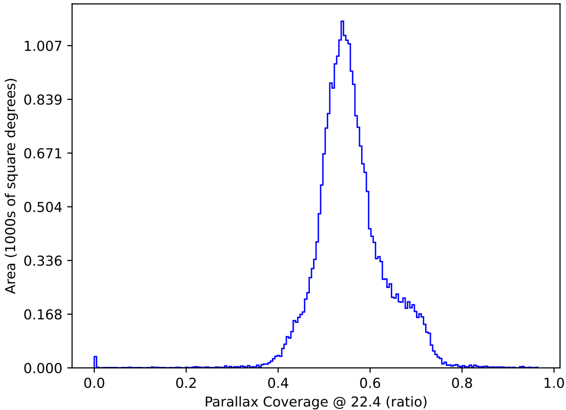
too_ignore_10_4v3.4_10yrs : Parallax Coverage @ 22.4
