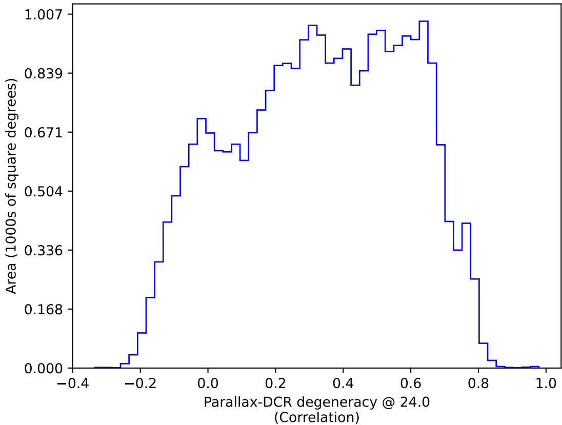
too_ignore_10_4v3.4_10yrs : Parallax-DCR degeneracy @ 24.0
