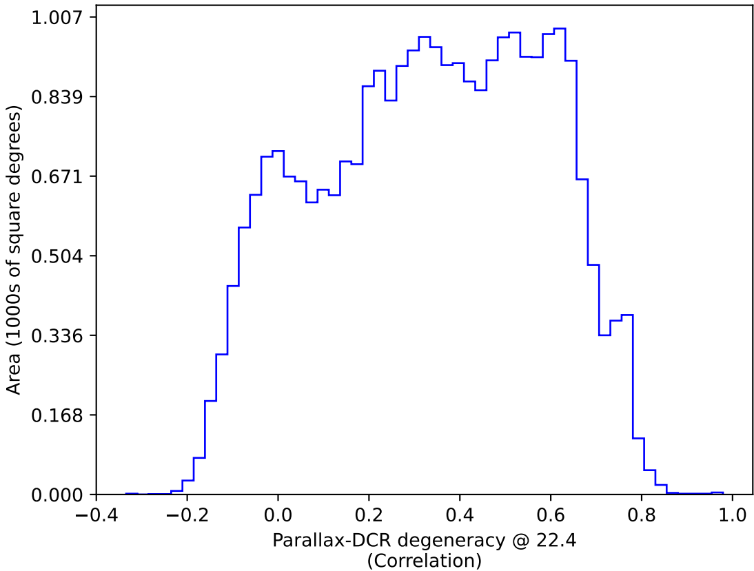
too_ignore_10_4v3.4_10yrs : Parallax-DCR degeneracy @ 22.4
