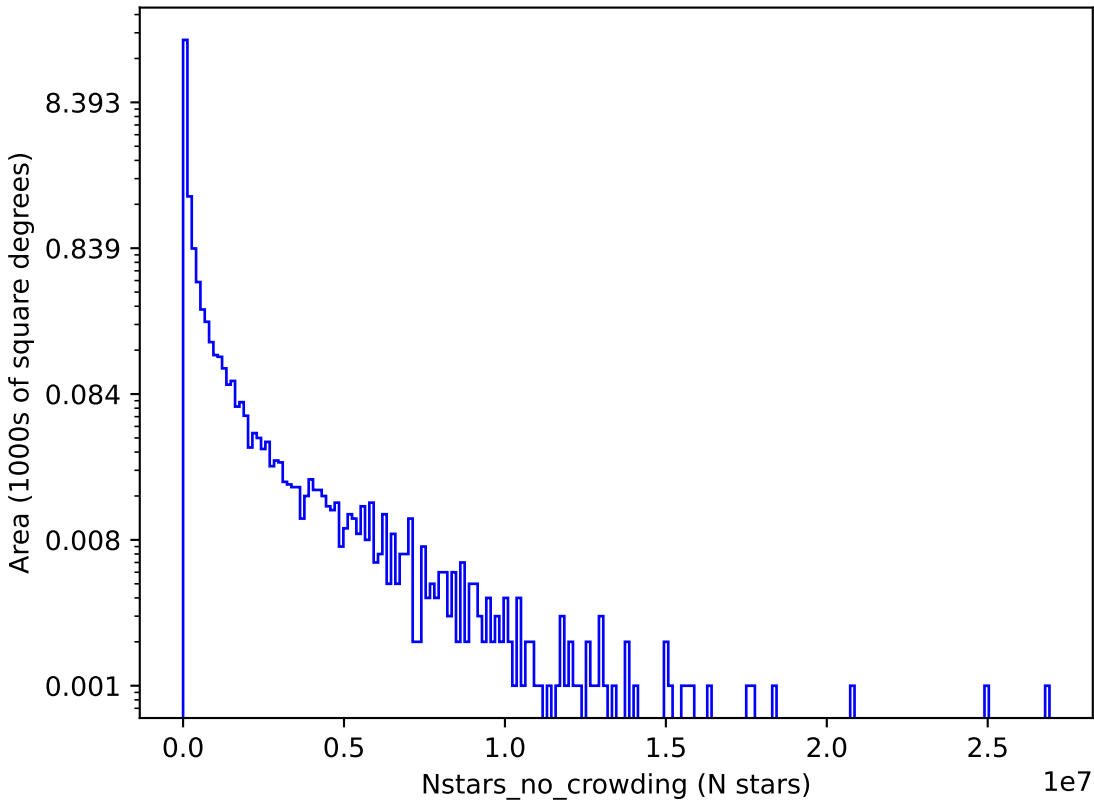
too_ignore_10_4v3.4_10yrs z: Nstars_no_crowding
