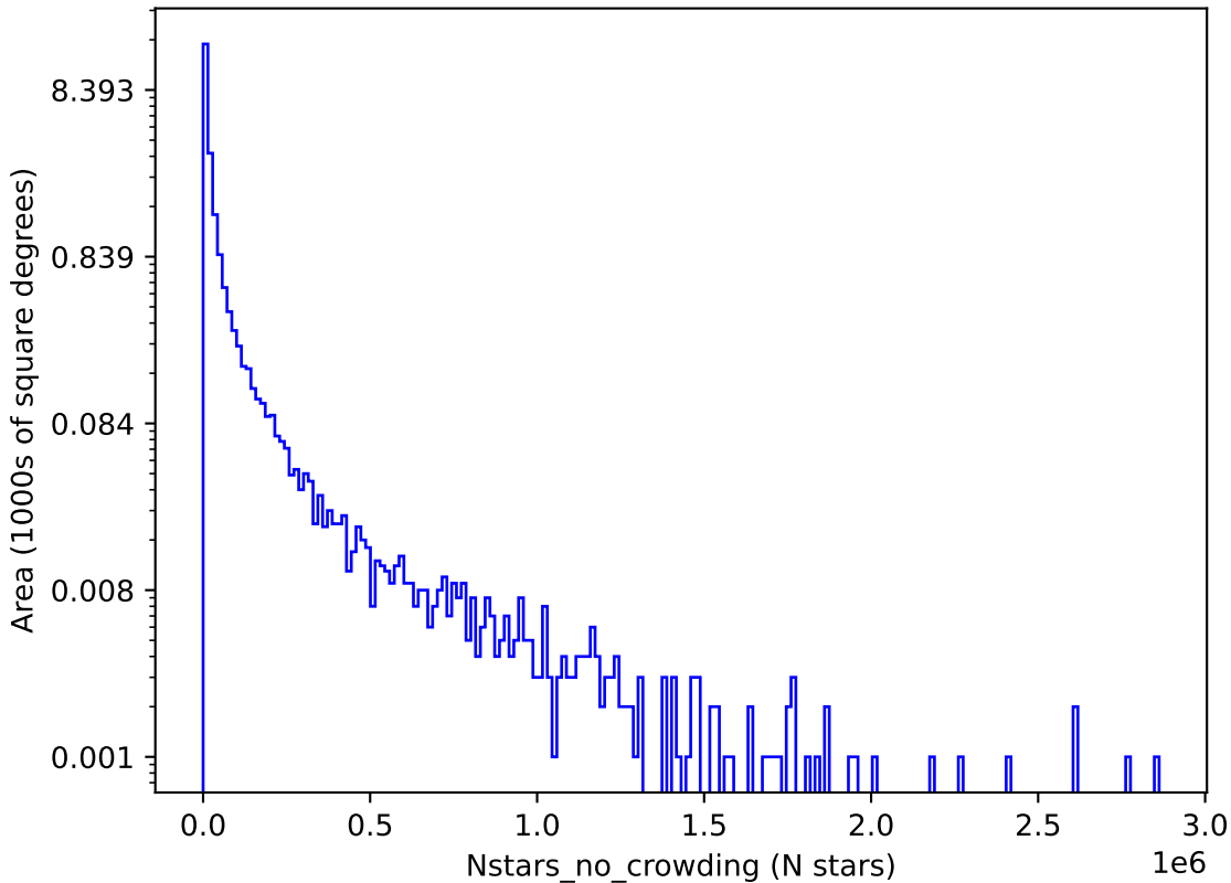
too_ignore_10_4v3.4_10yrs u: Nstars_no_crowding
