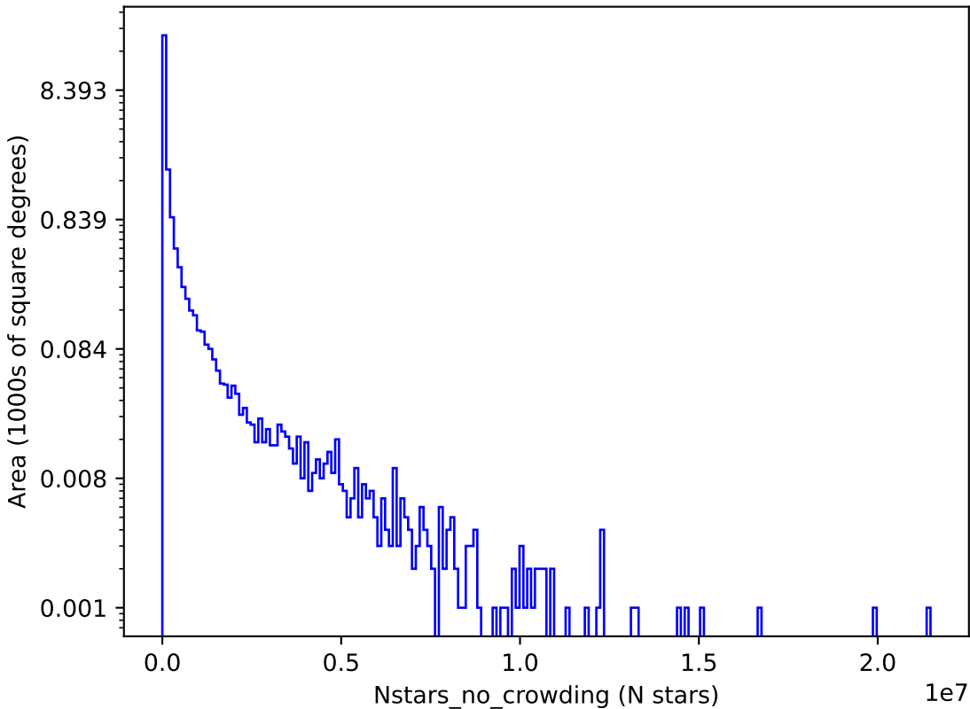
too_ignore_10_4v3.4_10yrs r: Nstars_no_crowding
