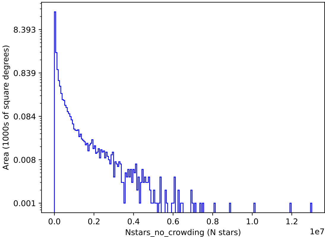
too_ignore_10_4v3.4_10yrs g: Nstars_no_crowding
