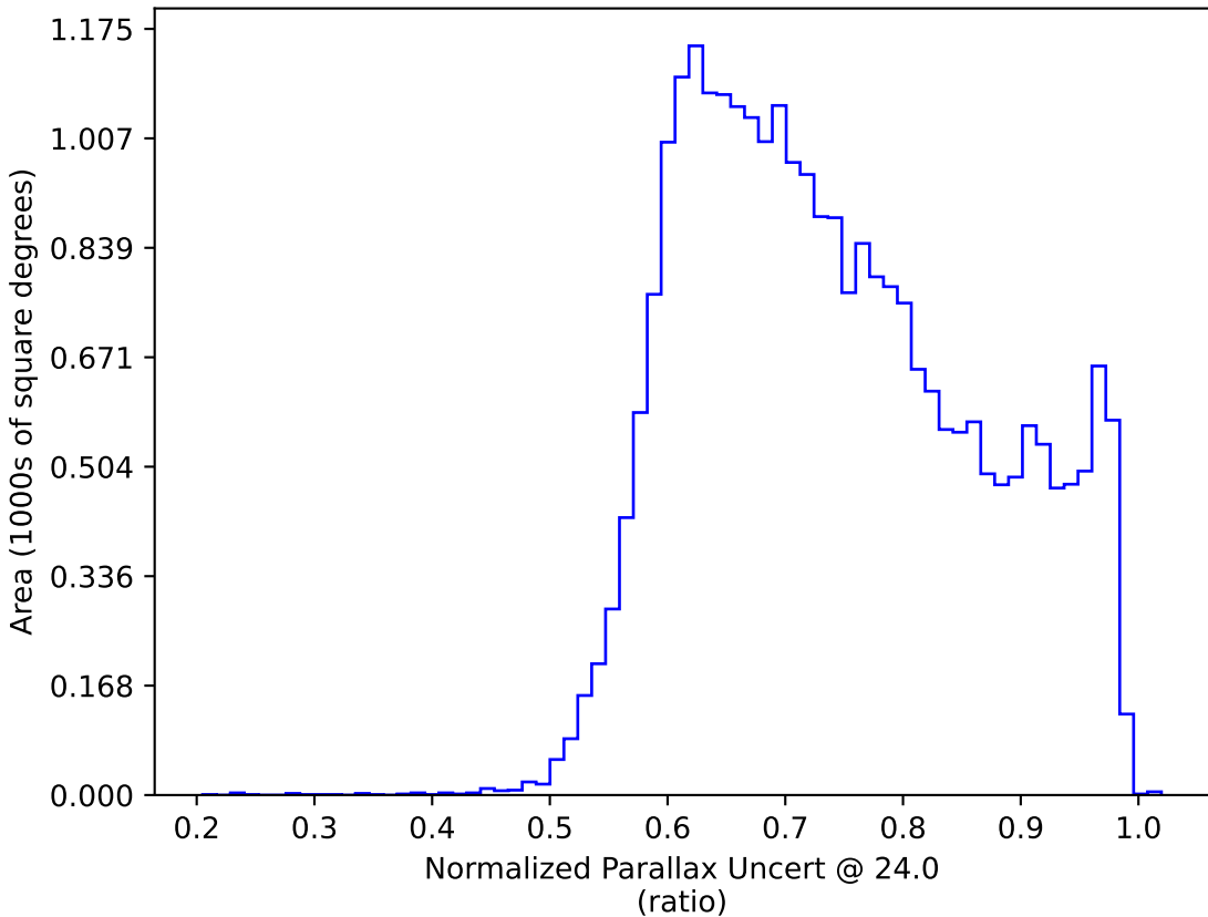
too_ignore_10_4v3.4_10yrs : Normalized Parallax Uncert @ 24.0
