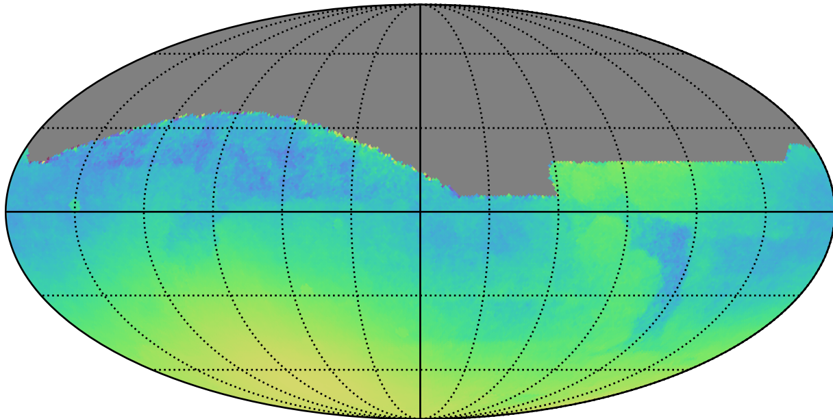
too_ignore_10_4v3.4_10yrs : Normalized Parallax Uncert @ 22.4
