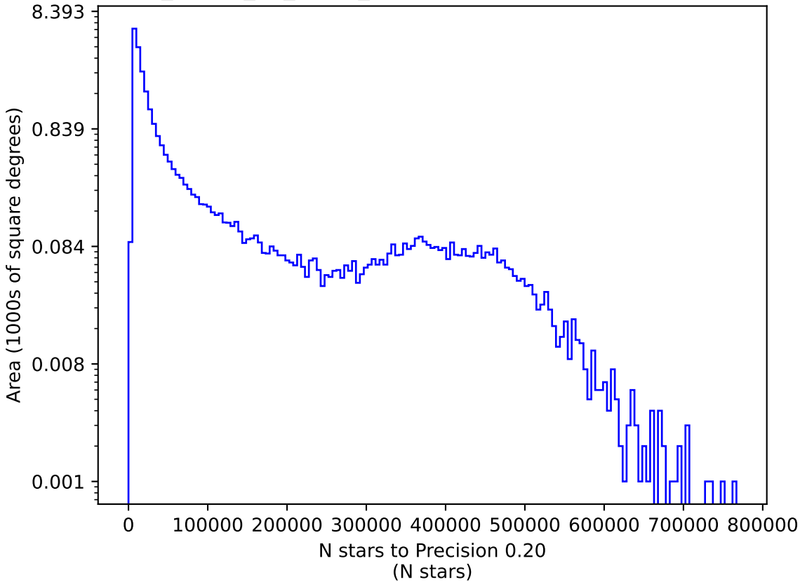
too_ignore_10_4v3.4_10yrs z: N stars to Precision 0.20
