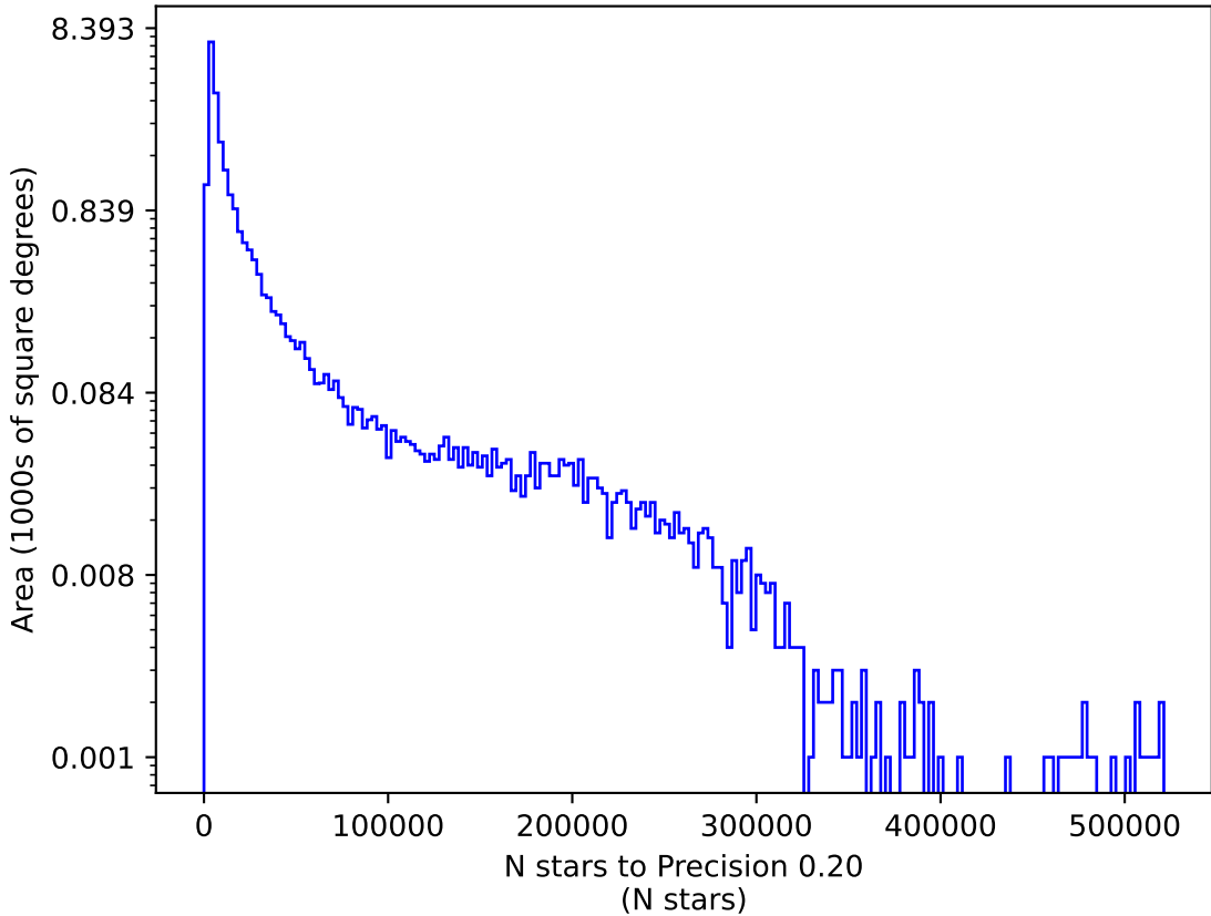
too_ignore_10_4v3.4_10yrs u: N stars to Precision 0.20
