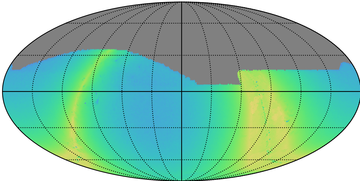
too_ignore_10_4v3.4_10yrs i: N stars to Precision 0.20
