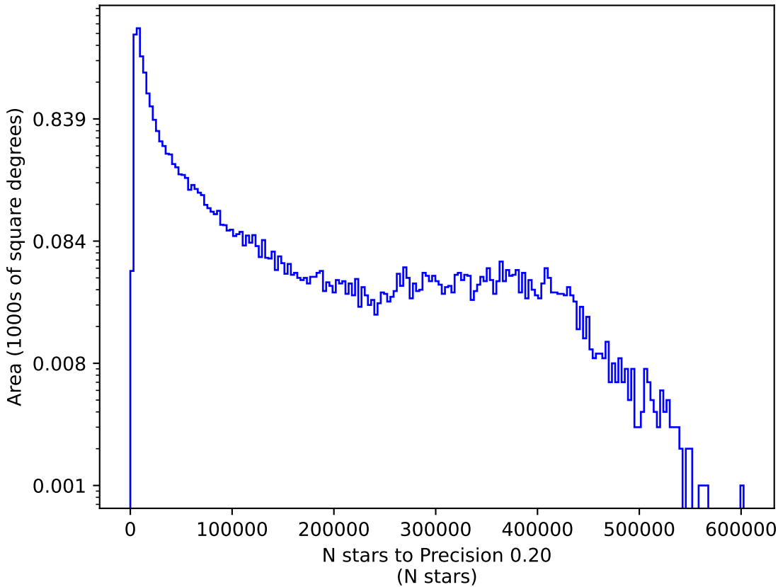
too_ignore_10_4v3.4_10yrs g: N stars to Precision 0.20
