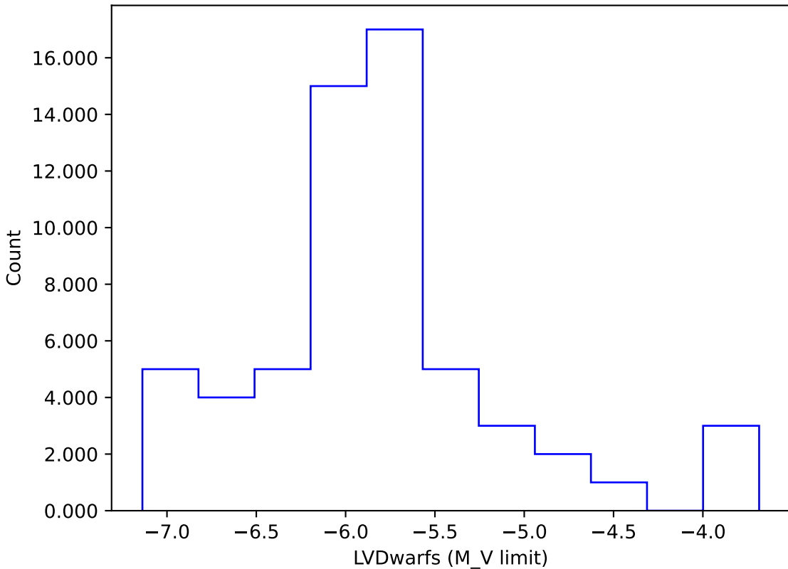
too_ignore_10_4v3.4_10yrs gi: LVDwarfs
