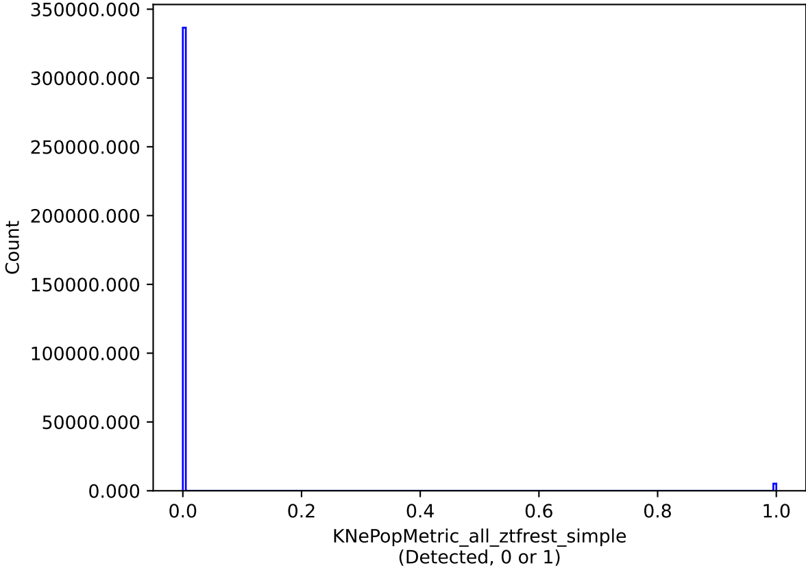
too_ignore_10_4v3.4_10yrs all models: KNePopMetric_all_ztfrest_simple
