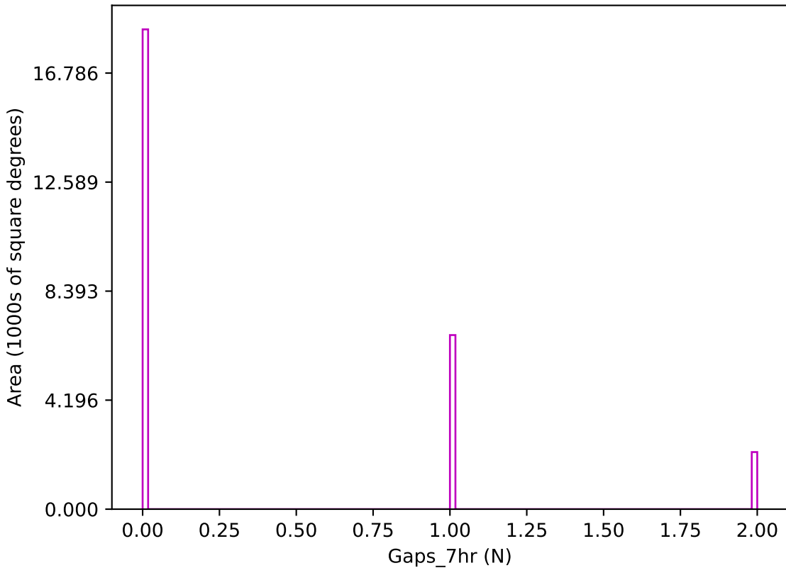
too_ignore_10_4v3.4_10yrs z band: Gaps_7hr
