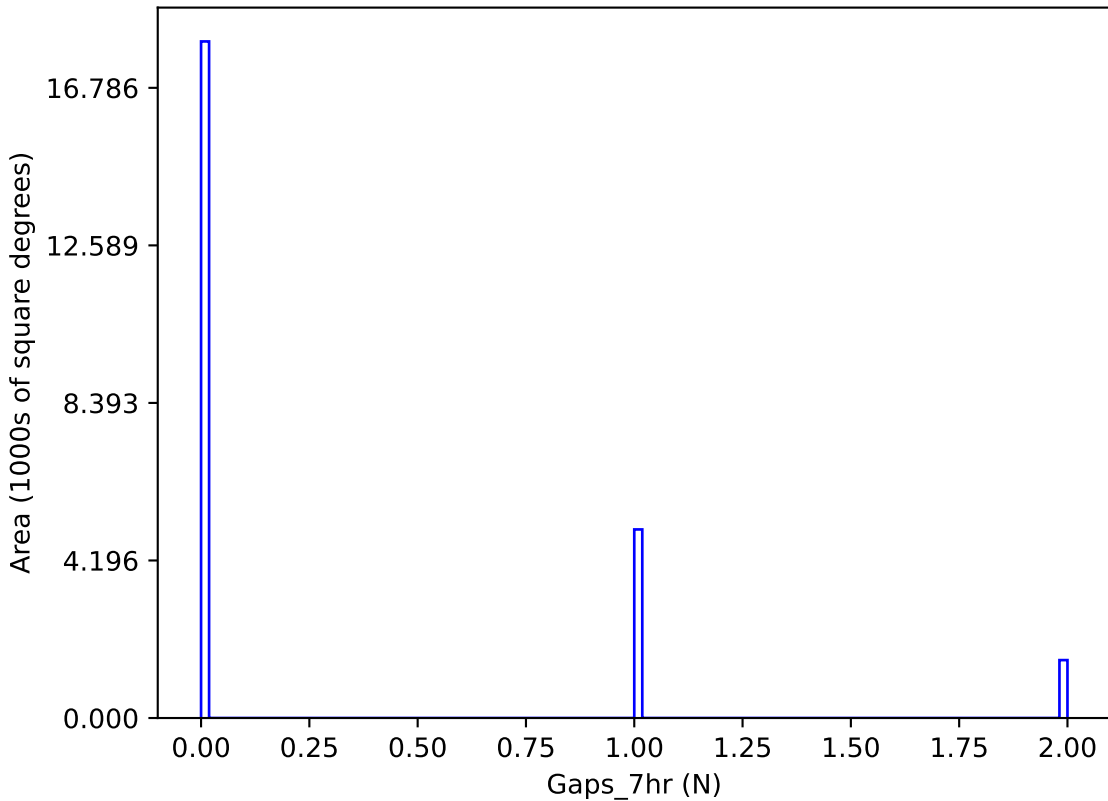
too_ignore_10_4v3.4_10yrs y band: Gaps_7hr
