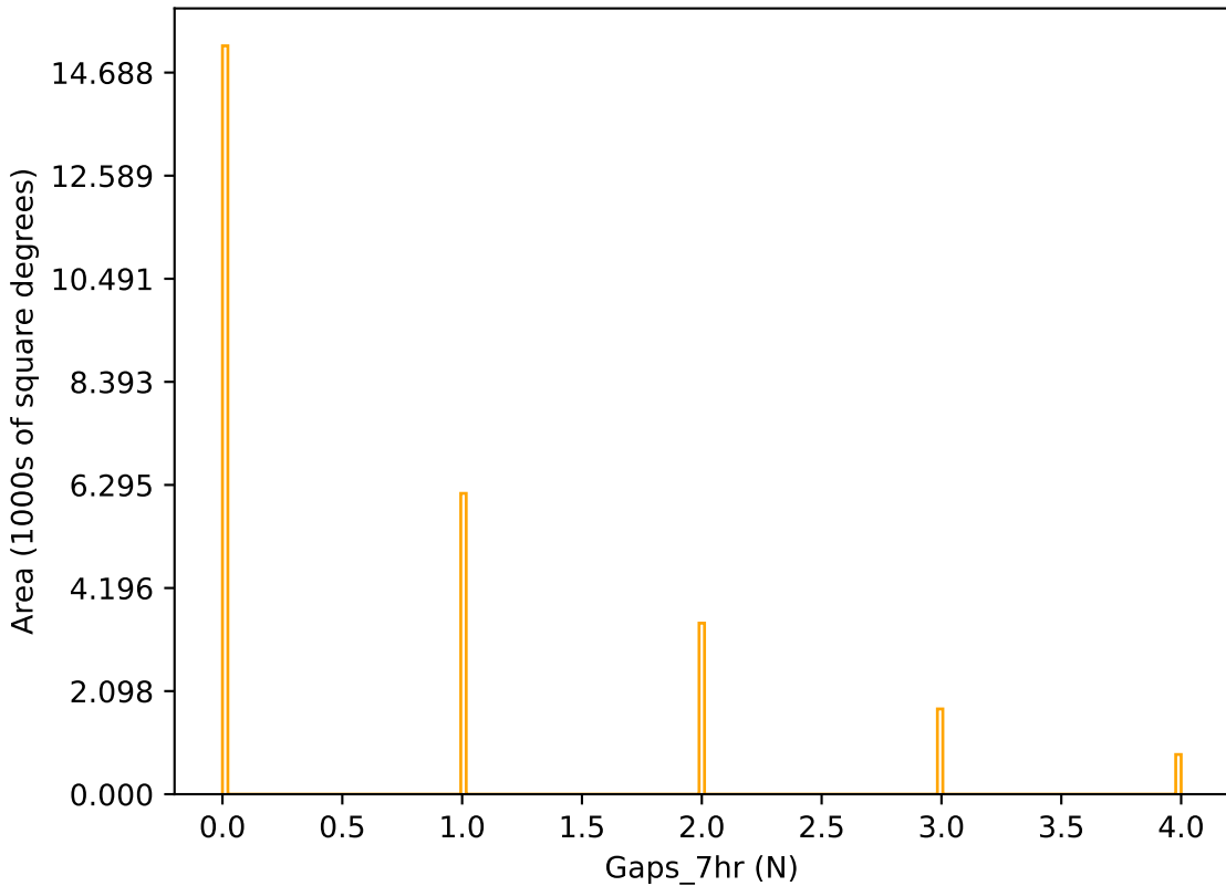
too_ignore_10_4v3.4_10yrs r band: Gaps_7hr
