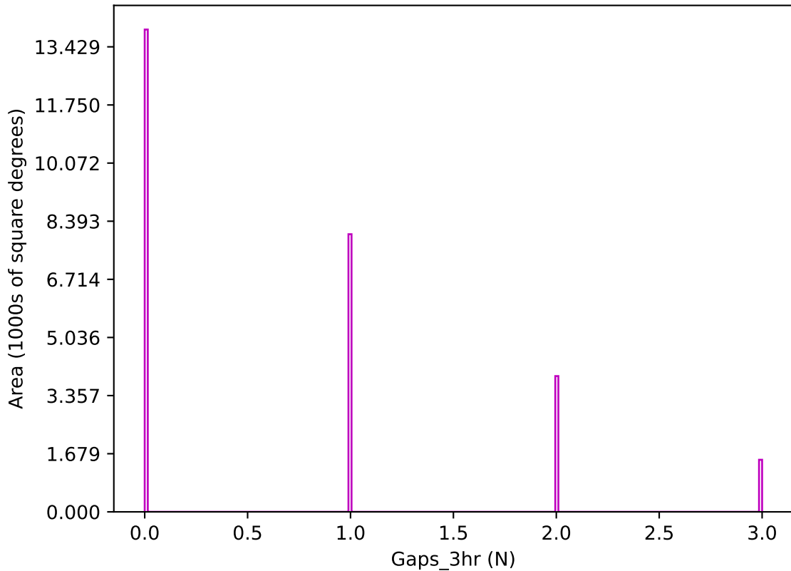
too_ignore_10_4v3.4_10yrs z band: Gaps_3hr
