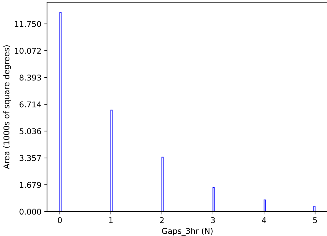
too_ignore_10_4v3.4_10yrs y band: Gaps_3hr
