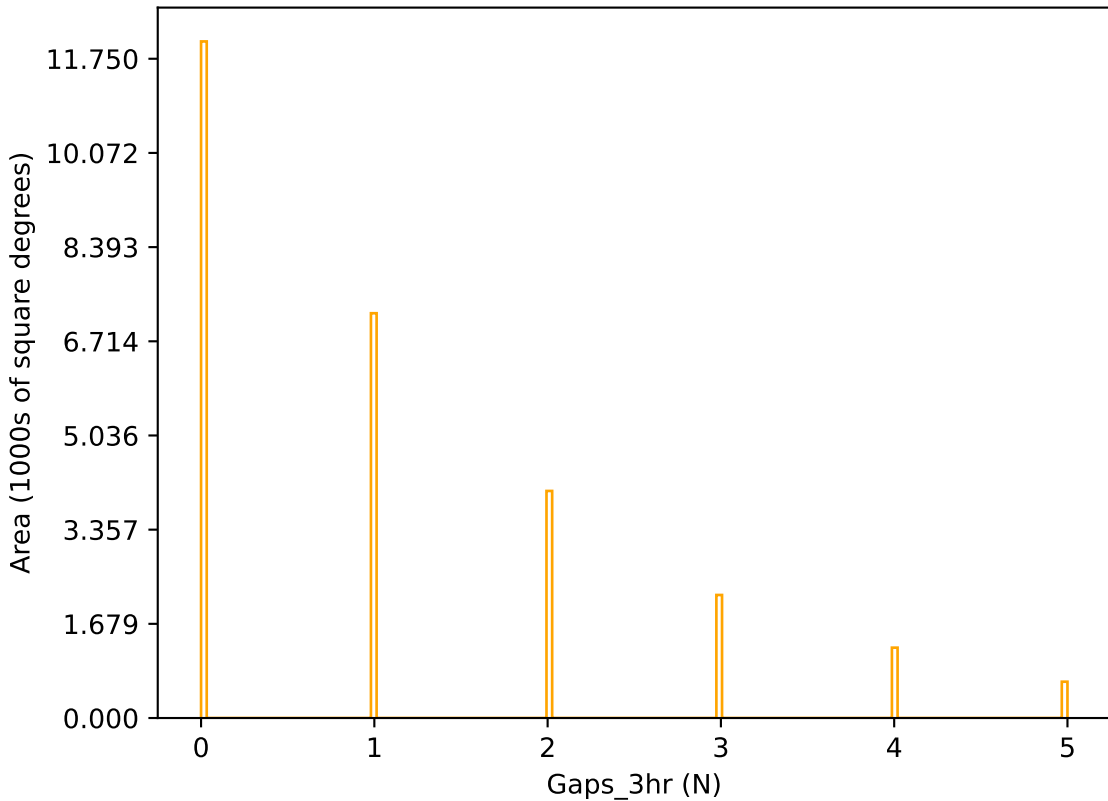
too_ignore_10_4v3.4_10yrs r band: Gaps_3hr
