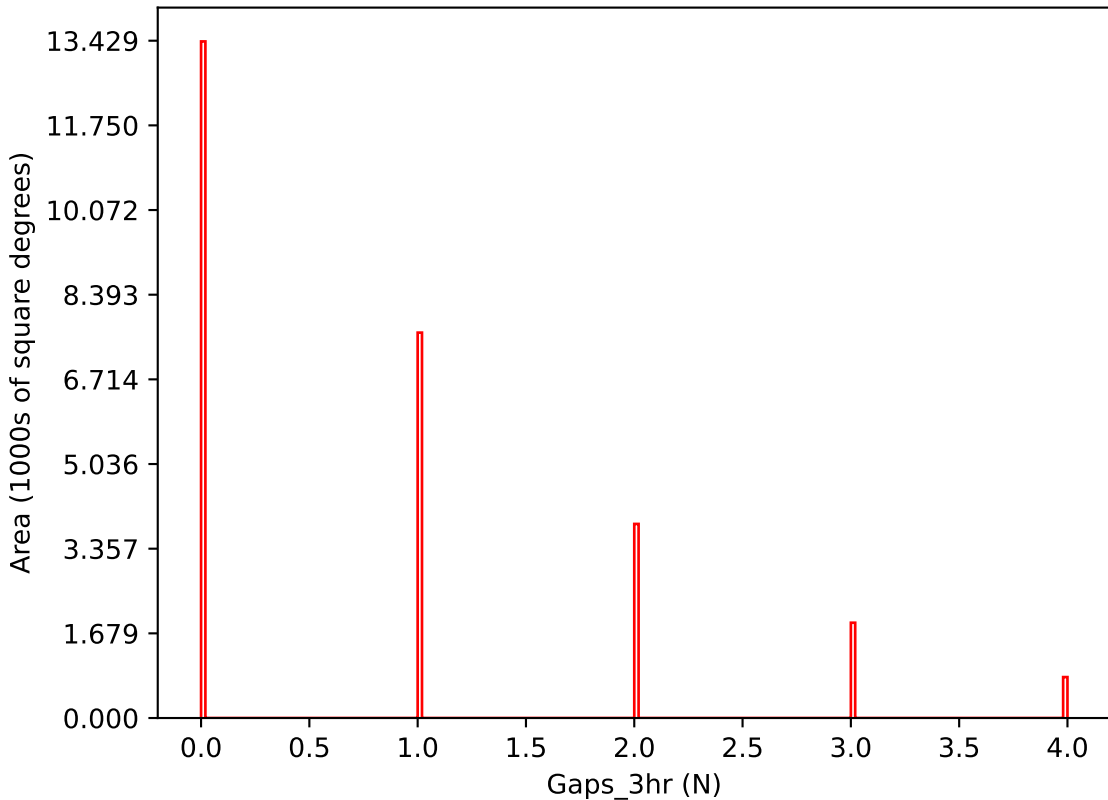
too_ignore_10_4v3.4_10yrs i band: Gaps_3hr
