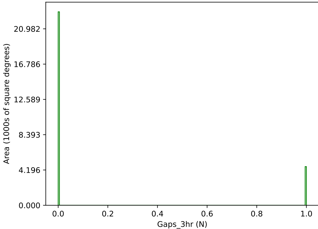
too_ignore_10_4v3.4_10yrs g band: Gaps_3hr
