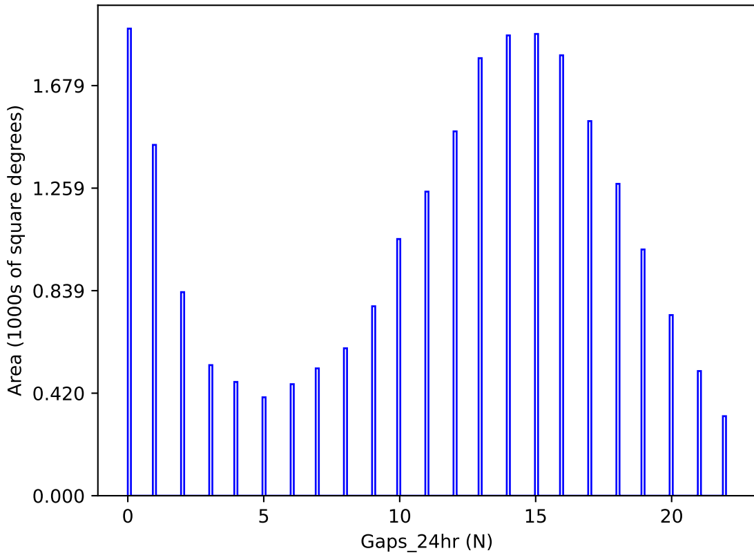
too_ignore_10_4v3.4_10yrs y band: Gaps_24hr
