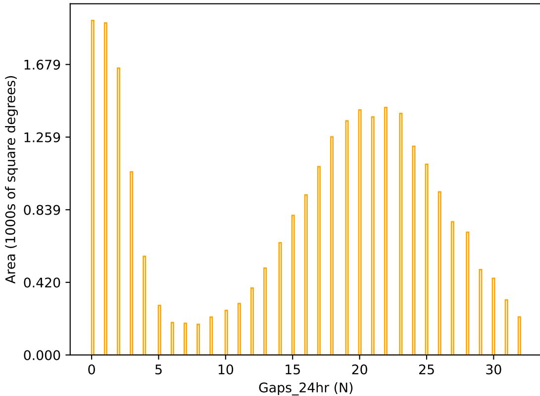
too_ignore_10_4v3.4_10yrs r band: Gaps_24hr
