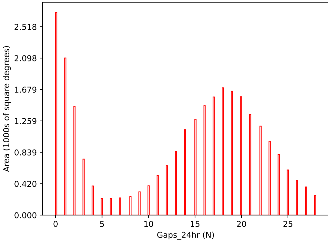
too_ignore_10_4v3.4_10yrs i band: Gaps_24hr
