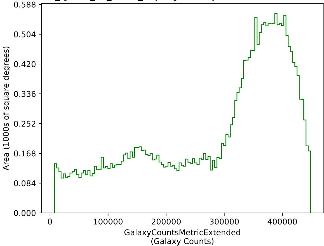
too_ignore_10_4v3.4_10yrs g: GalaxyCountsMetricExtended
