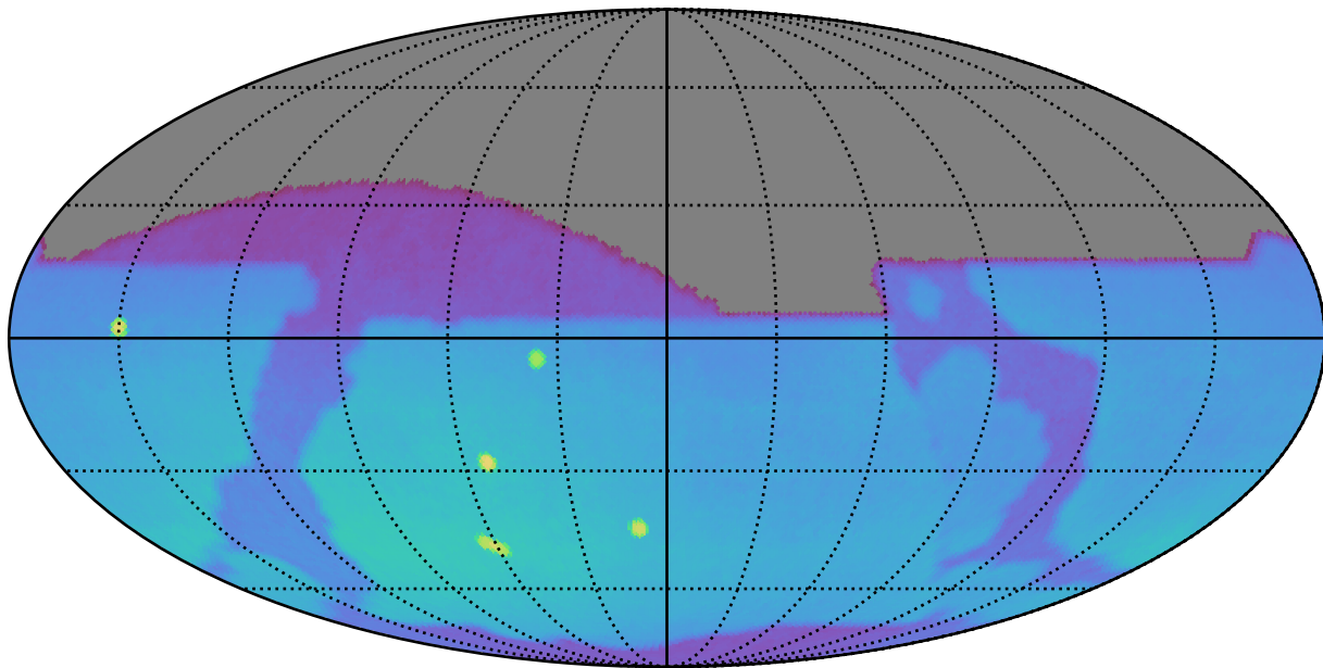
too_ignore_10_4v3.4_10yrs : Brown Dwarf, L4
