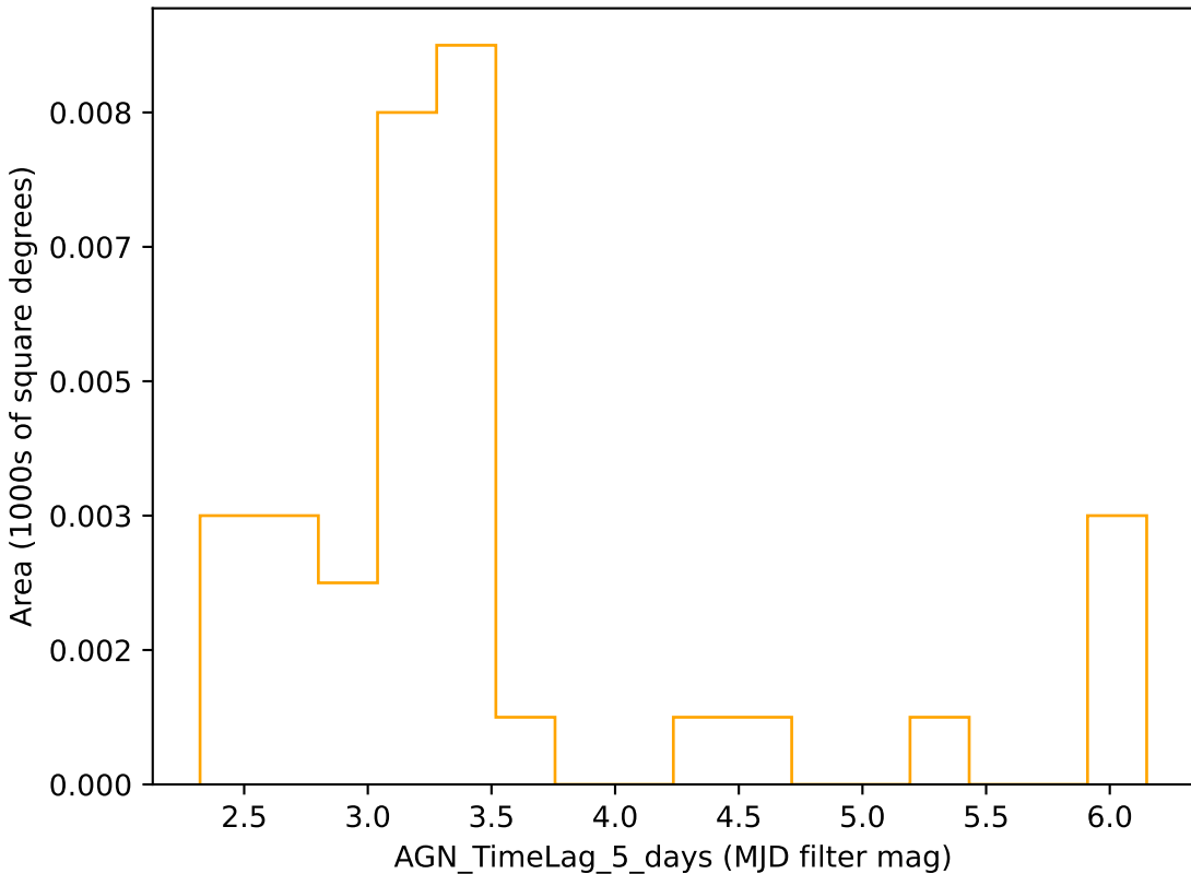
too_ignore_10_4v3.4_10yrs r band: AGN_TimeLag_5_days
