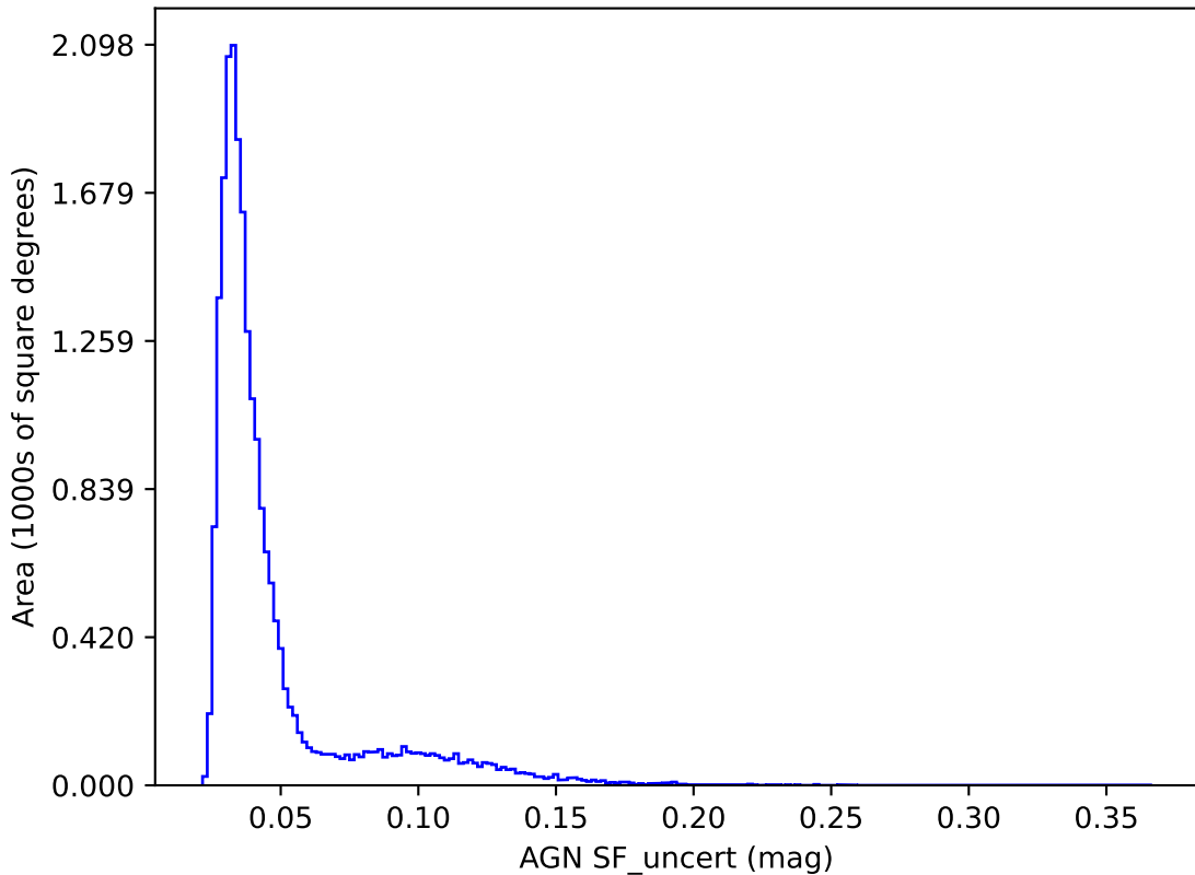
too_ignore_10_4v3.4_10yrs y band: AGN SF_uncert
