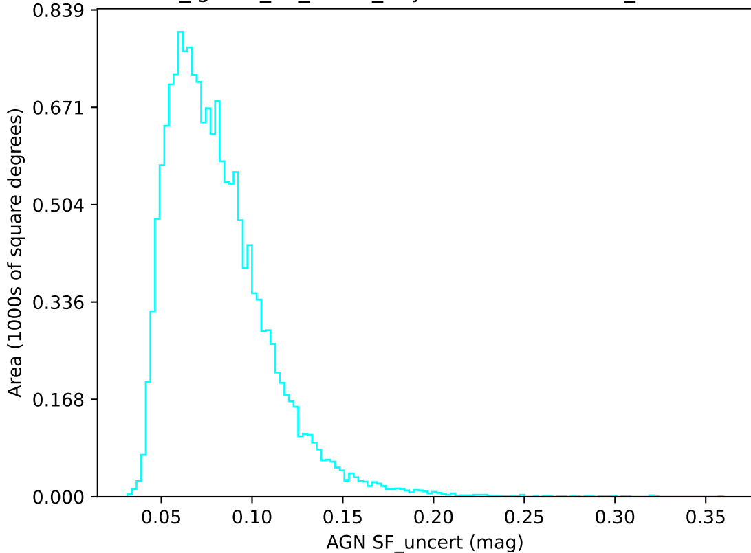
too_ignore_10_4v3.4_10yrs u band: AGN SF_uncert
