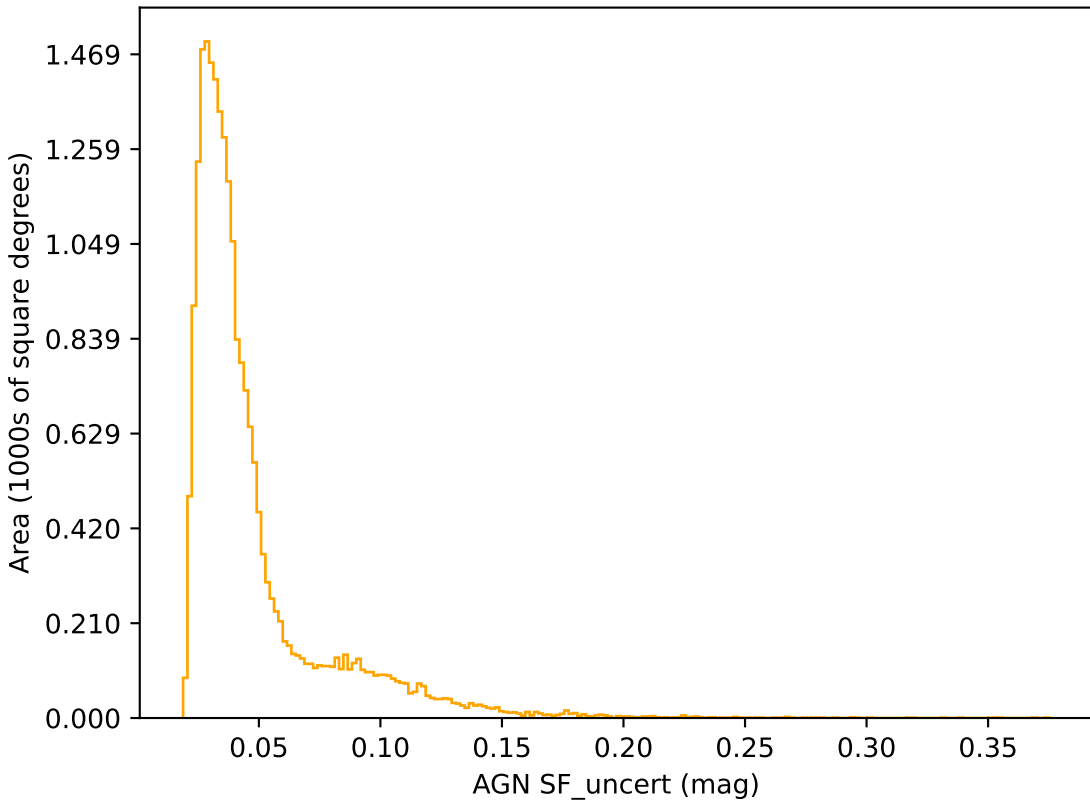
too_ignore_10_4v3.4_10yrs r band: AGN SF_uncert
