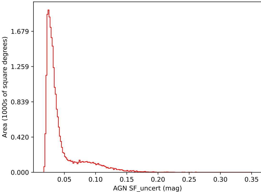
too_ignore_10_4v3.4_10yrs i band: AGN SF_uncert
