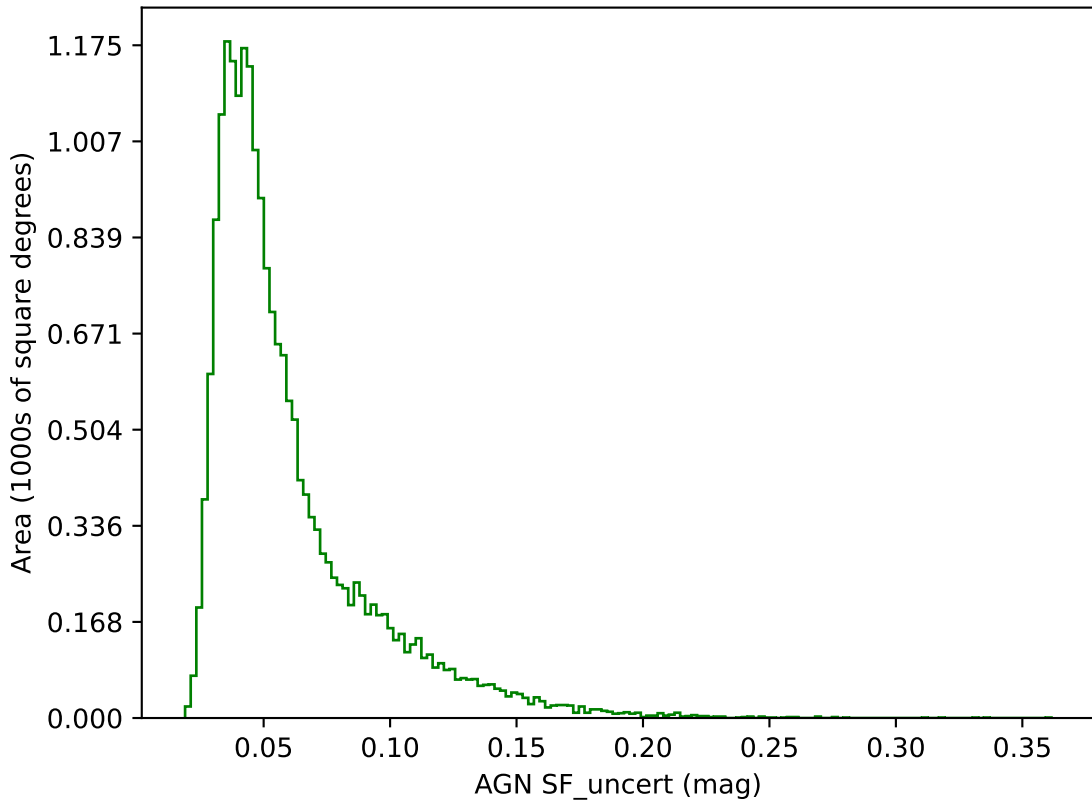
too_ignore_10_4v3.4_10yrs g band: AGN SF_uncert
