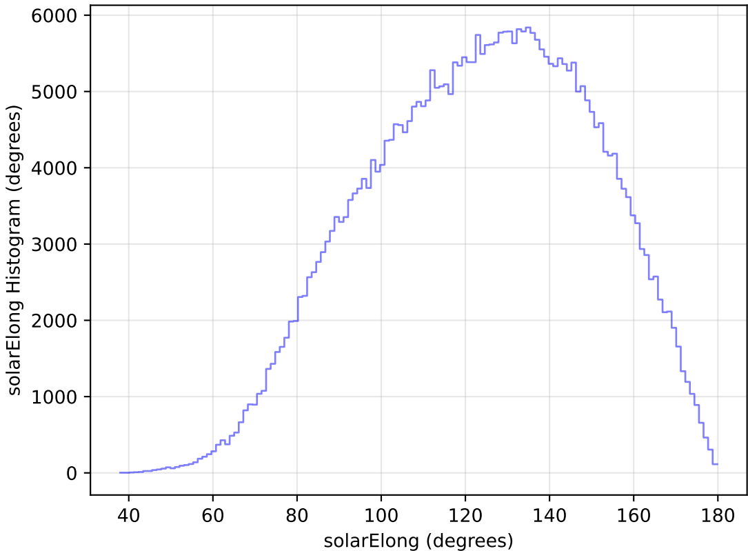
too_ignore_10_4v3.4_10yrs WFD y band: solarElong Histogram
