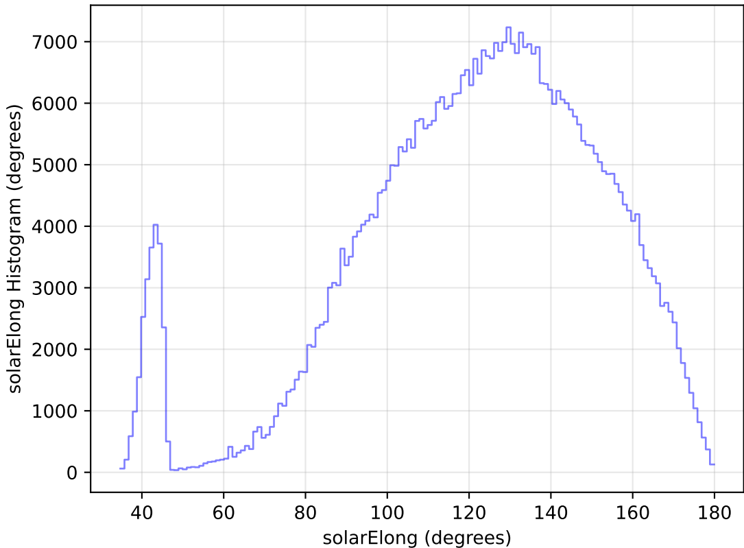
too_ignore_10_4v3.4_10yrs WFD i band: solarElong Histogram
