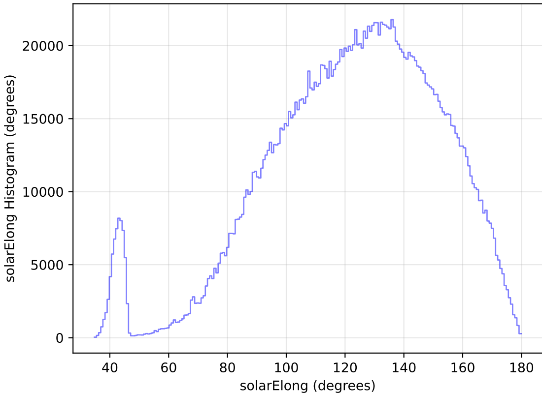
too_ignore_10_4v3.4_10yrs WFD all bands: solarElong Histogram
