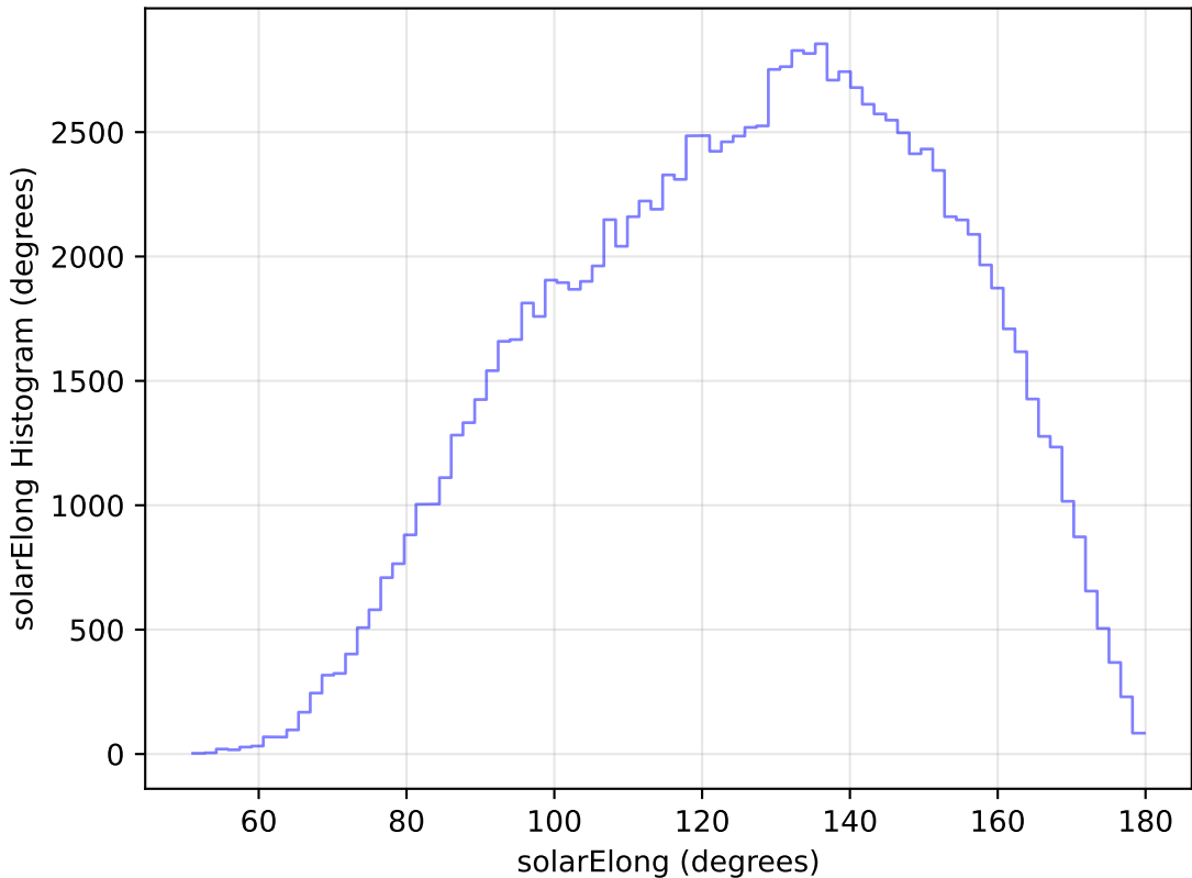
too_ignore_10_4v3.4_10yrs All sky u band: solarElong Histogram
