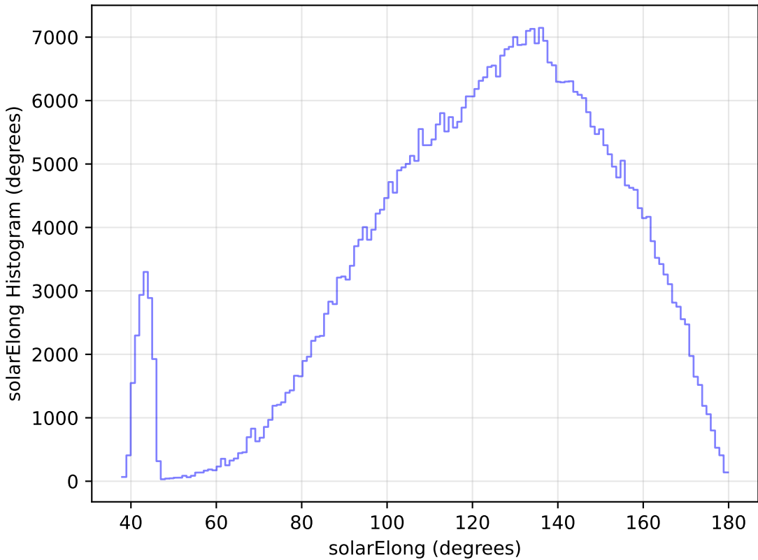
too_ignore_10_4v3.4_10yrs All sky r band: solarElong Histogram
