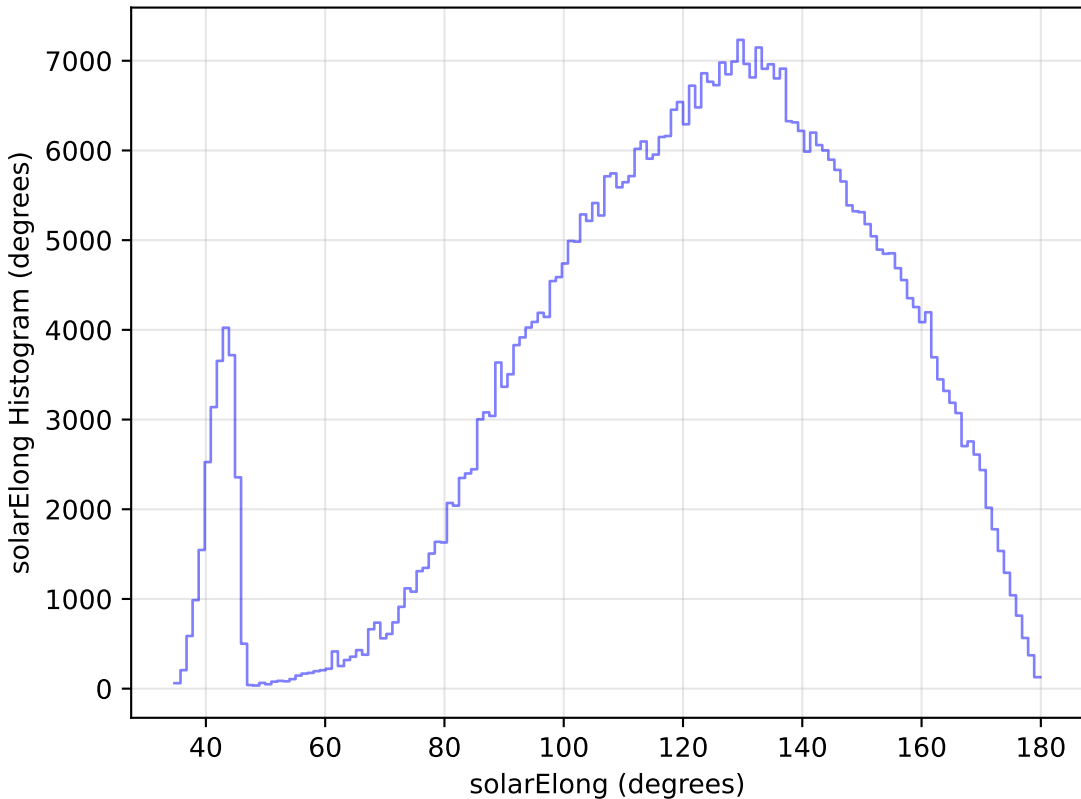
too_ignore_10_4v3.4_10yrs All sky i band: solarElong Histogram
