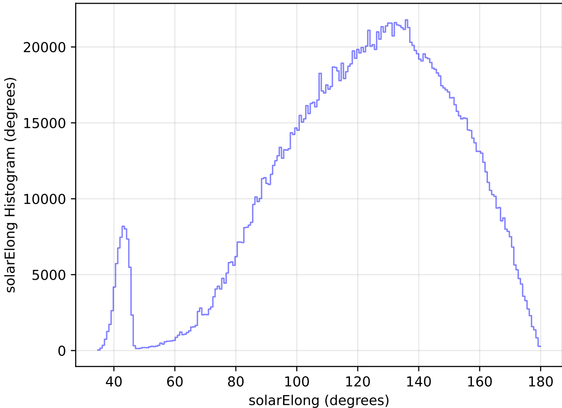
too_ignore_10_4v3.4_10yrs All sky all bands: solarElong Histogram
