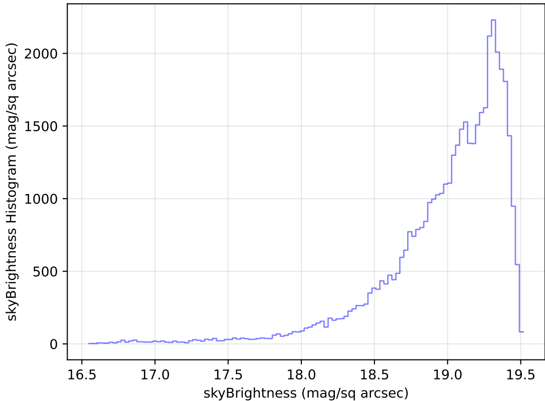
too_ignore_10_4v3.4_10yrs Yr 1 z band: skyBrightness Histogram
