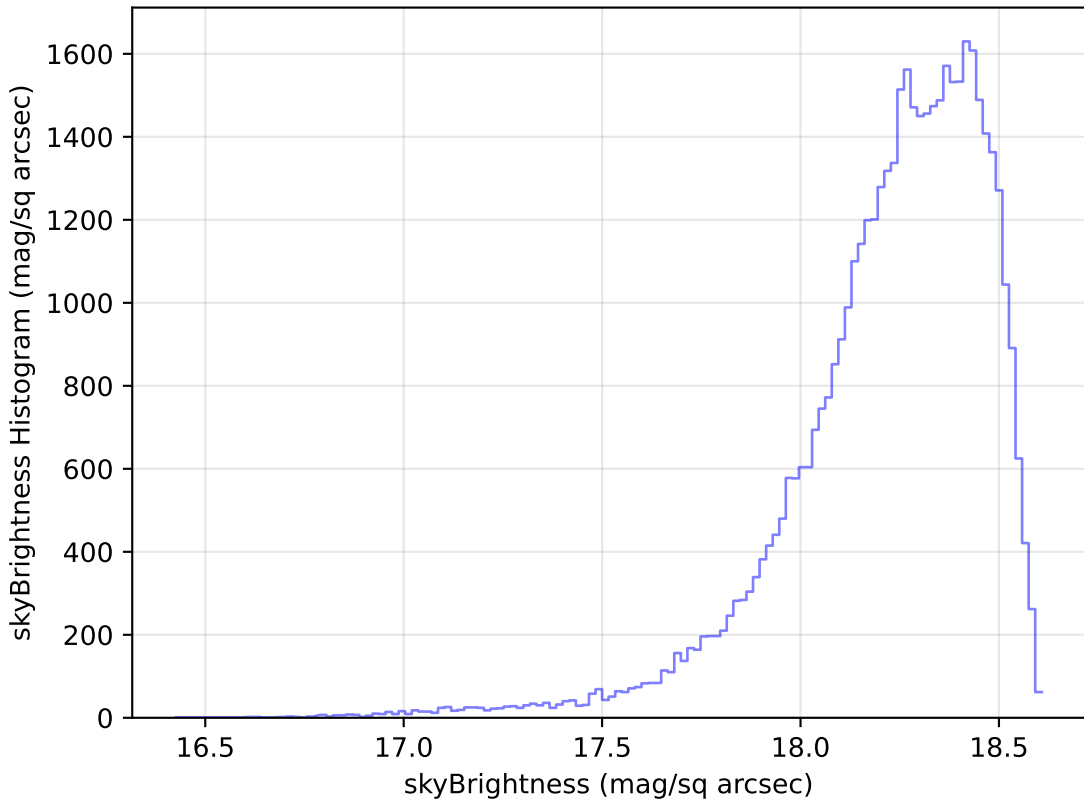
too_ignore_10_4v3.4_10yrs Yr 1 y band: skyBrightness Histogram
