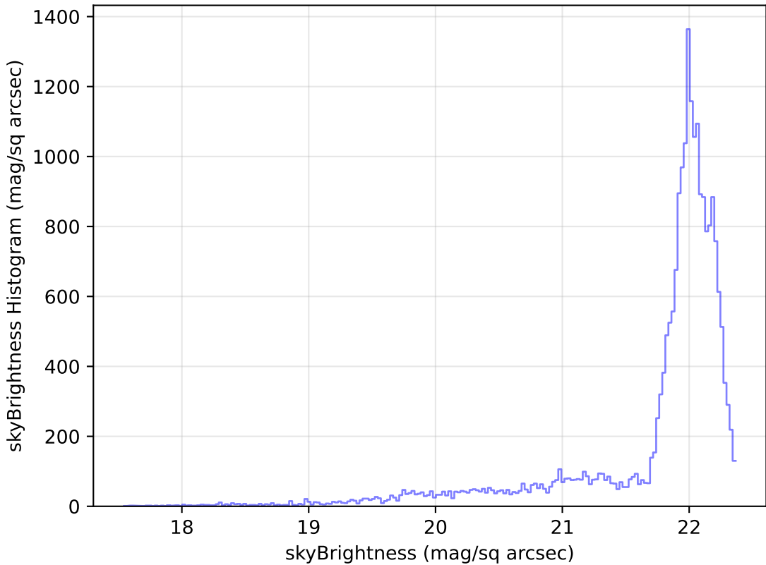
too_ignore_10_4v3.4_10yrs Yr 1 g band: skyBrightness Histogram
