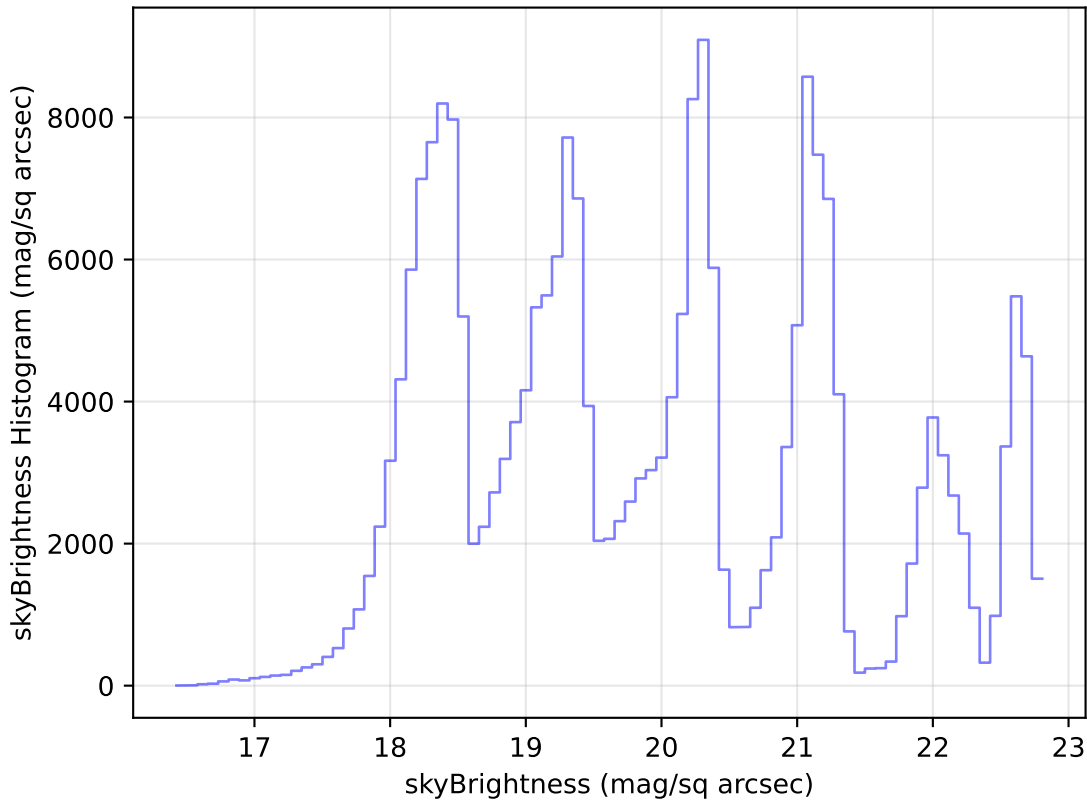
too_ignore_10_4v3.4_10yrs Yr 1 all bands: skyBrightness Histogram
