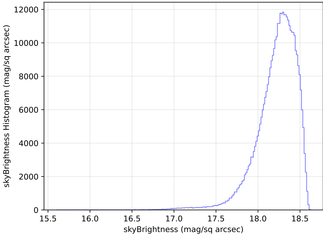
too_ignore_10_4v3.4_10yrs WFD y band: skyBrightness Histogram
