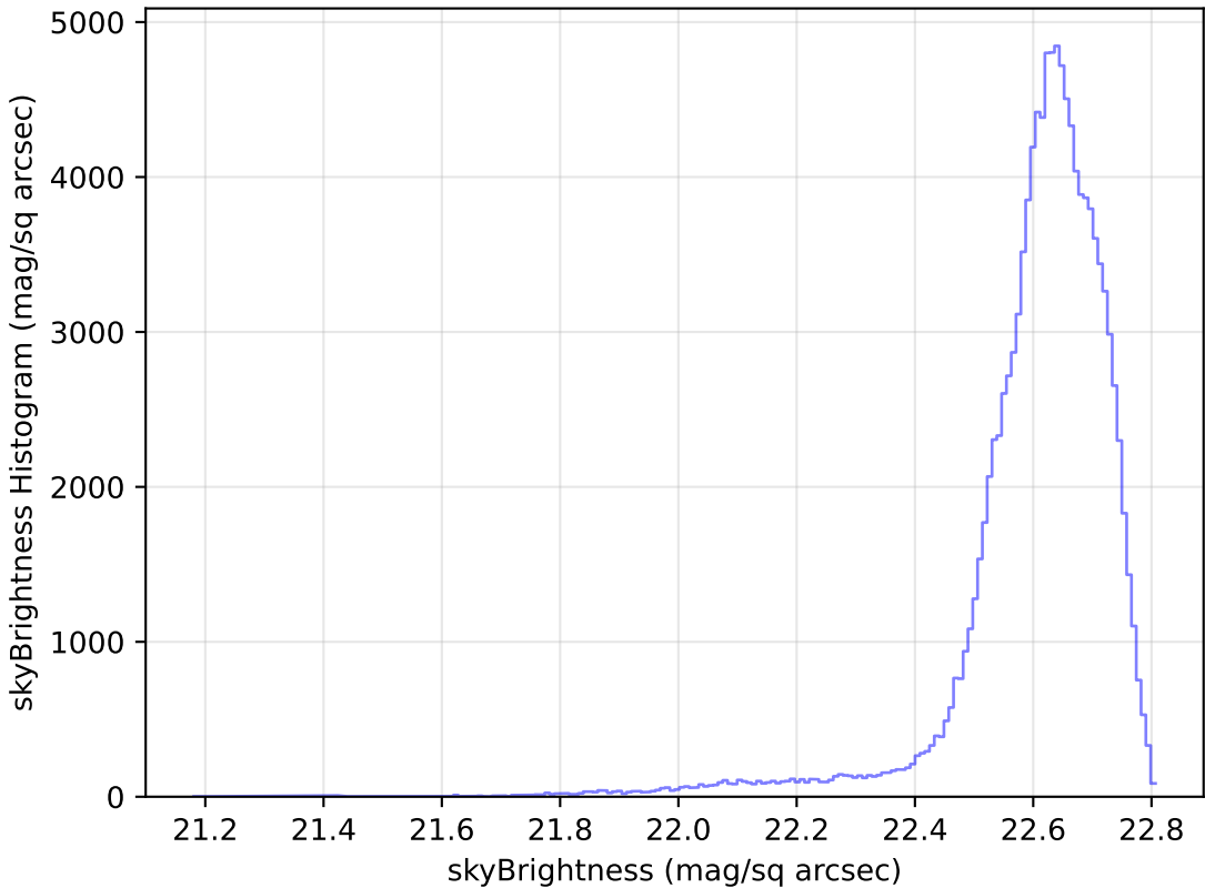
too_ignore_10_4v3.4_10yrs WFD u band: skyBrightness Histogram
