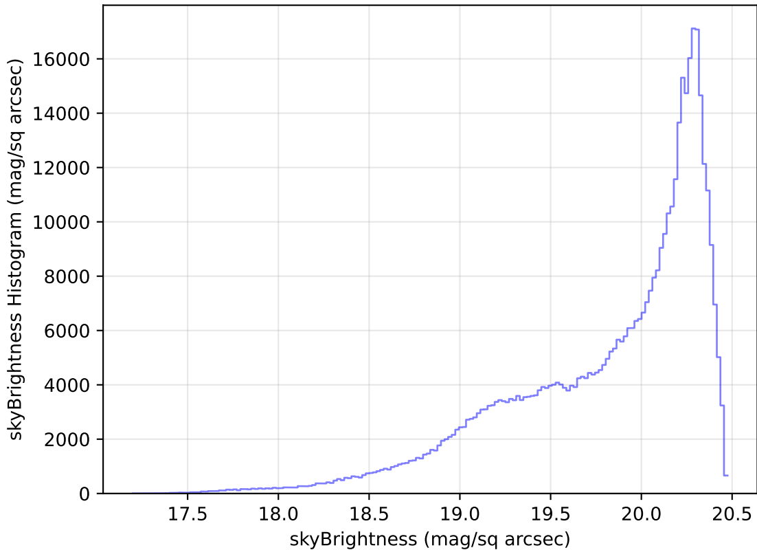
too_ignore_10_4v3.4_10yrs WFD i band: skyBrightness Histogram
