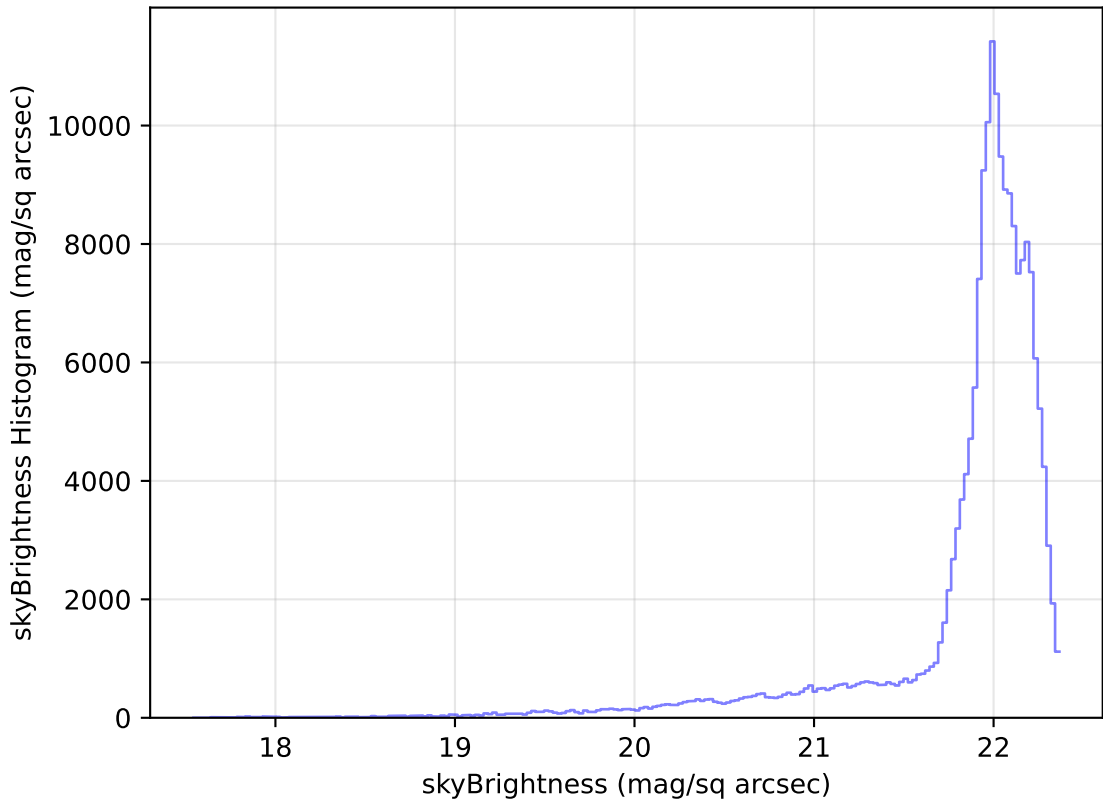
too_ignore_10_4v3.4_10yrs WFD g band: skyBrightness Histogram
