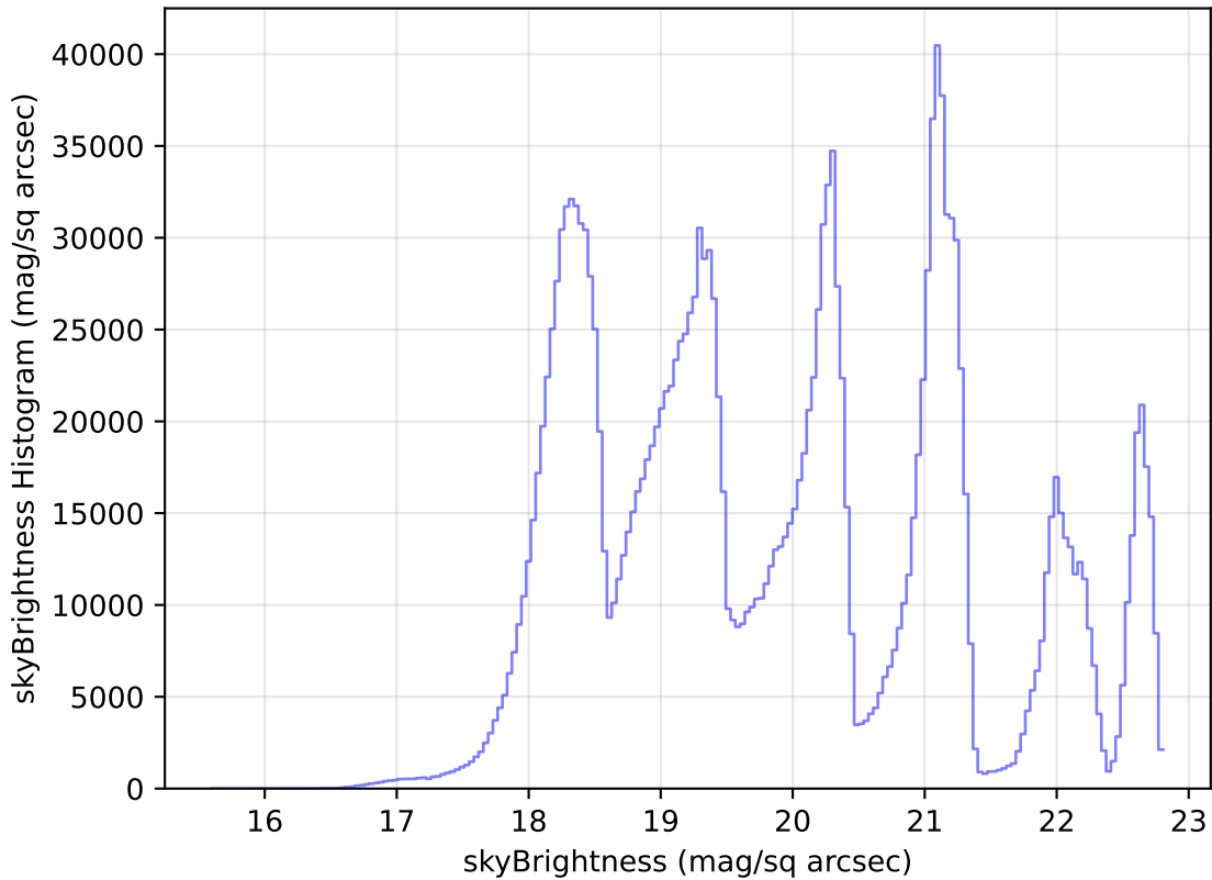
too_ignore_10_4v3.4_10yrs WFD all bands: skyBrightness Histogram
